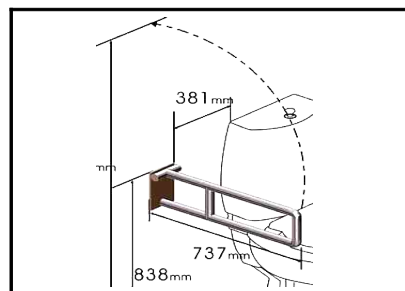
RR [ IMPORT ] BNH - 9032 Swing-up support rail 800 x 32
