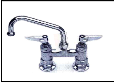
T & S [ USA ] RB - 0225-062X 4" Centers deck mixing faucet c/w 12" swing nozzle
