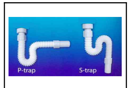
RR [ LOCAL ] RWT - 002 1 1/2" Uni-trap [ flexible bend ]
