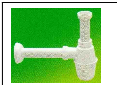
RR [ LOCAL ] RPM - 3106 1 1/4" Plastic bottle trap IN WHITE
