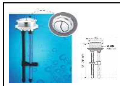
RR [ LOCAL ] RTP - 1042 Dual flush top push round button in 48mm
