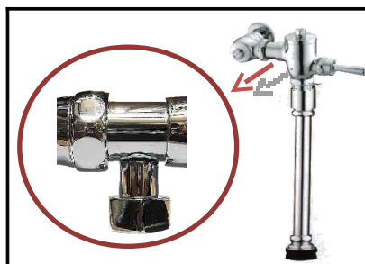
RR [ IMPORT ] RCH - B 06-1 WB - A WC Flush valve ( A type ) c/w F 1/2" connection for angle valve to bidet spray
