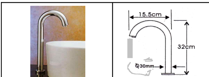
RR [ IMPORT ] RCH - F 910-32 Basin Faucet High Spout Automatic Sensor ( Battery operated )
