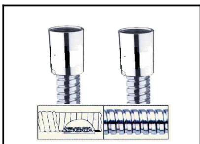
RST [ GERMANY ] RST - 1567 AGRAFF shower hose 2.0m Brass chrome-plated
